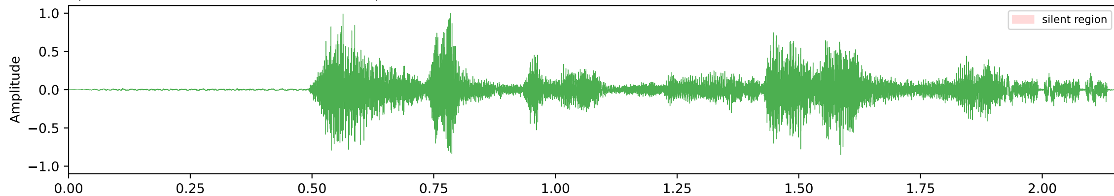
(C) Oracle-separated Speaker 2 (pro_006) — CATASTROPHIC HALLUCINATION Leading silence → Whisper enters token-id repetition loop: CER = 24.25, CR = 16.33 (transcript 24× longer than reference!)
