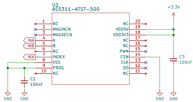
Incremental Magnetic Linear Encoder
