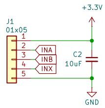
Armature Connection
