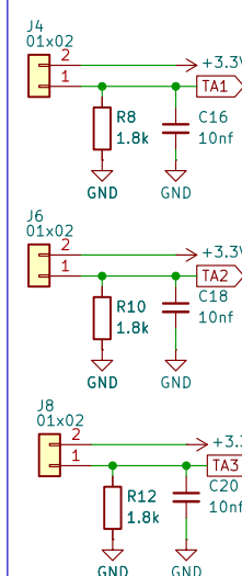
Thermistor Array (10k NTC) TA1-TA3
