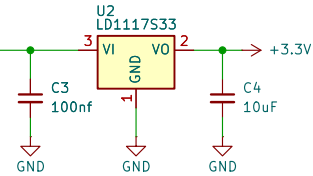
Low Dropout Regulator (5V to 3.3V)
