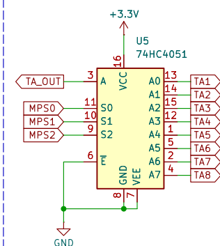
Thermistor Array Multiplexer
