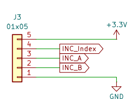
Linear Encoder Interconnect
