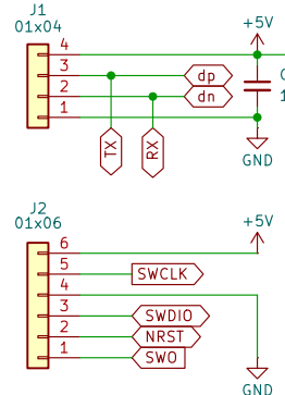
Driver Interconnect &amp; Serial Debug
