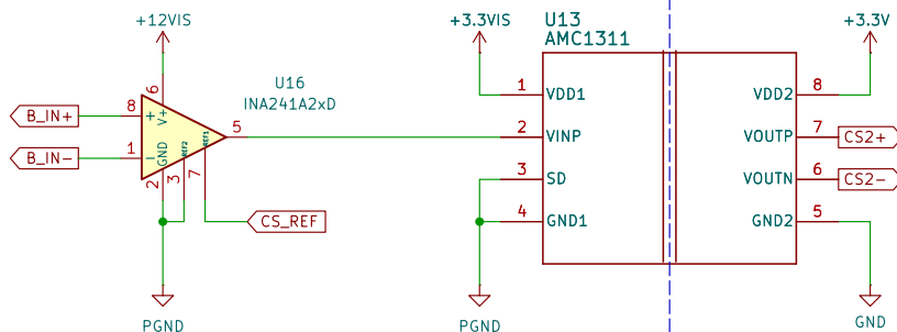
Current Sensor (Phase B)
