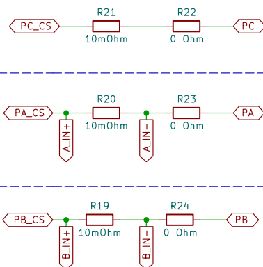
Phase Connections (upto 5.0 A (PEAK))
