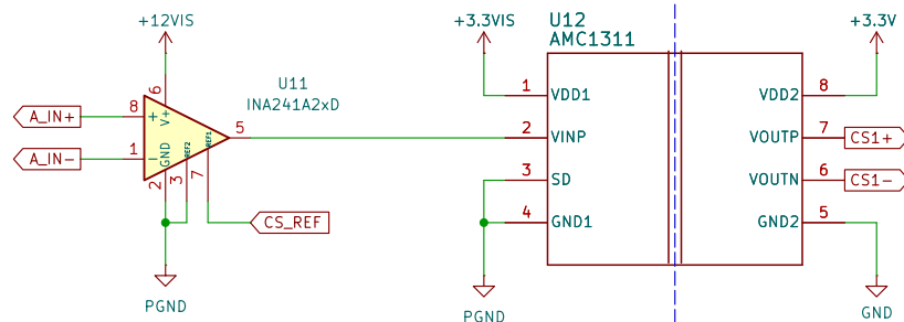
Current Sensor (Phase A)
