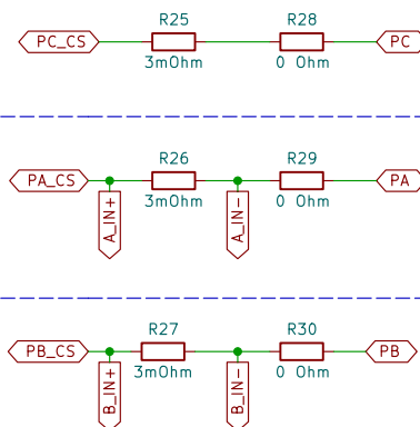
Phase Connections (upto 16.6 A (PEAK))
