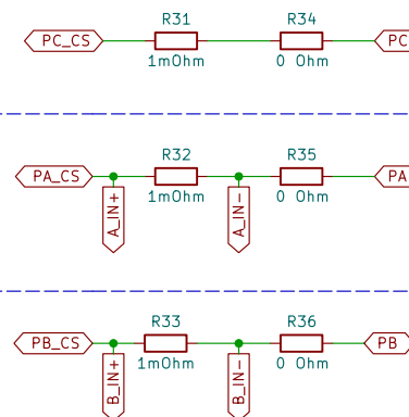
Phase Connections (upto 30 A (PEAK))
