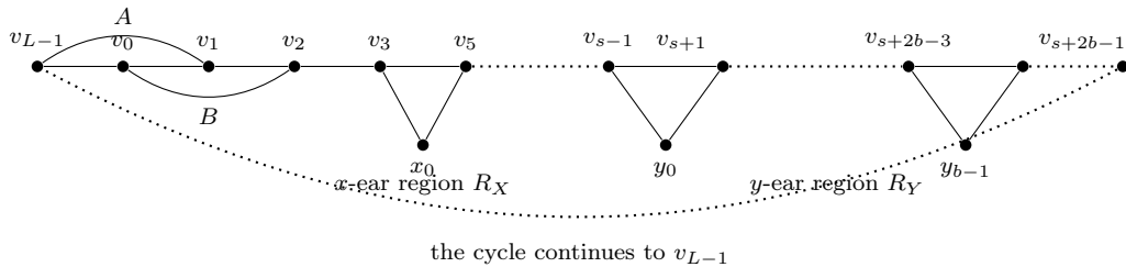
Figure 1: Schematic construction of G_{a,b}(L) . The graph consists of a long cycle, two short chords A and B , and two separated ear regions.
