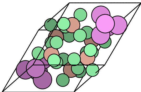
\text{Bi}_{10}\text{Cl}_{24}\text{Ga}_6
