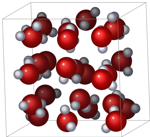
\text{H}_{54}\text{O}_{27}
