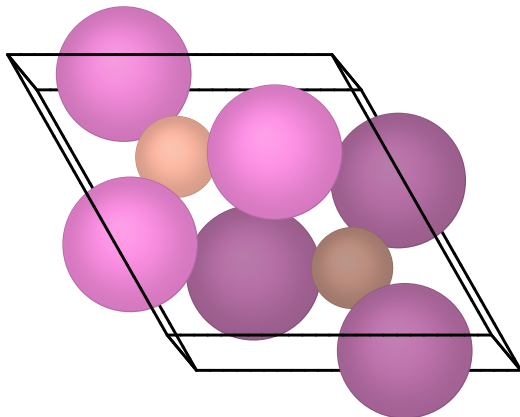
B2I6
