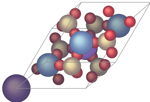
Na2O24P6Sn4
