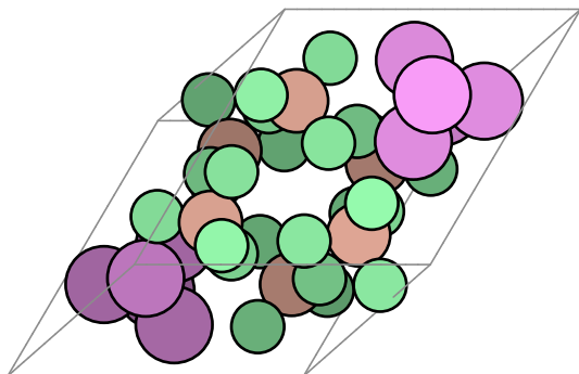
Bi10Cl24Ga6
