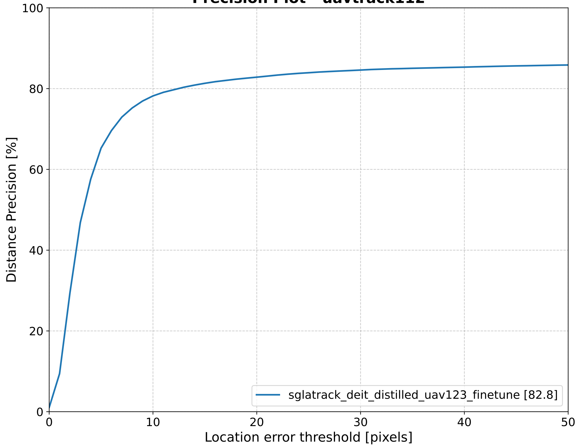
Precision Plot - uavtrack112
