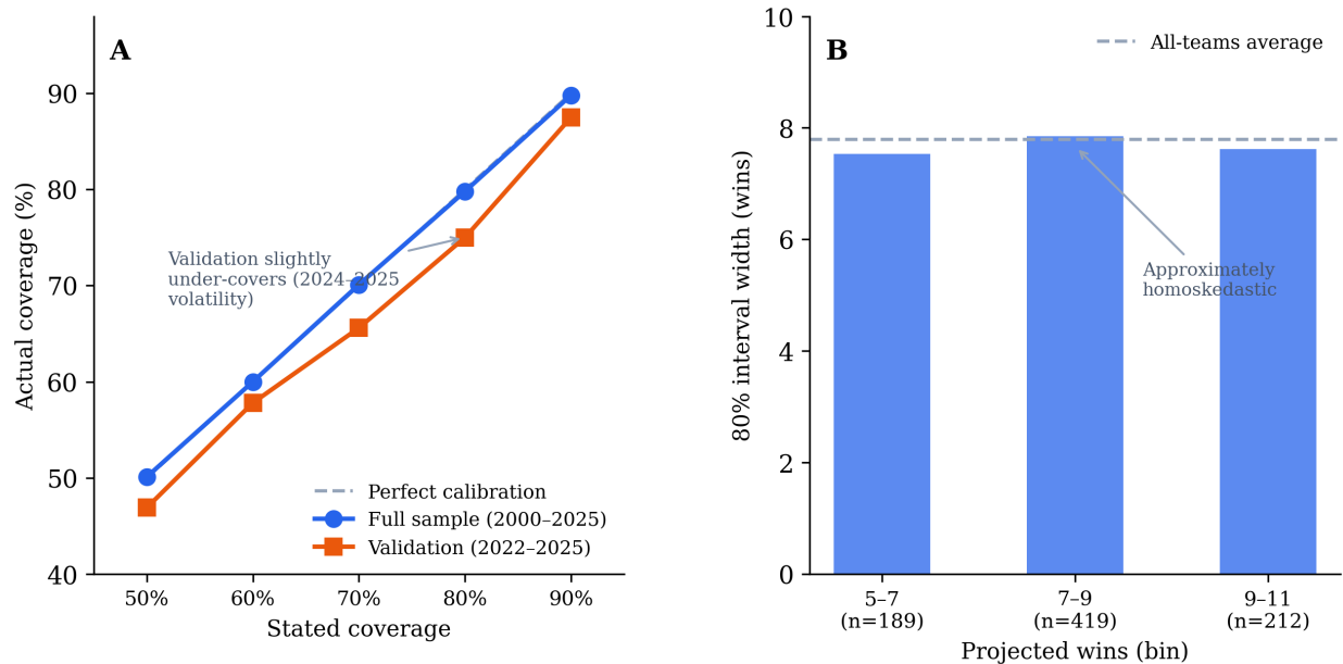
Figure 3: Figure 3. Prediction interval calibration. Panel A: stated vs actual coverage using leave-year-out residuals (full sample: near-perfect; validation 2022–2025: slight under-coverage consistent with elevated recent volatility). Panel B: 80% interval width by projection bin — approximately flat across the projection range.
