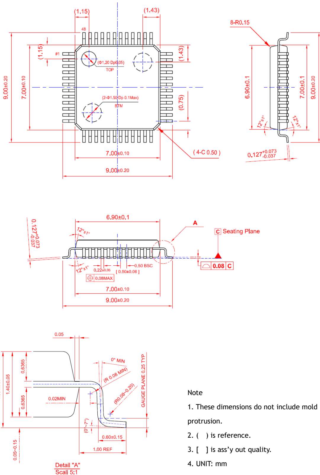
Figure 27. Package Dimensions
