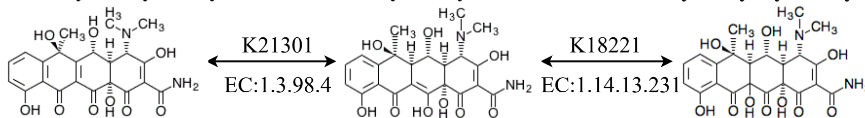
5a,11a-Dehydroxytetracycline
