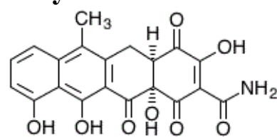
4-Keto-anhydrotetracycline
