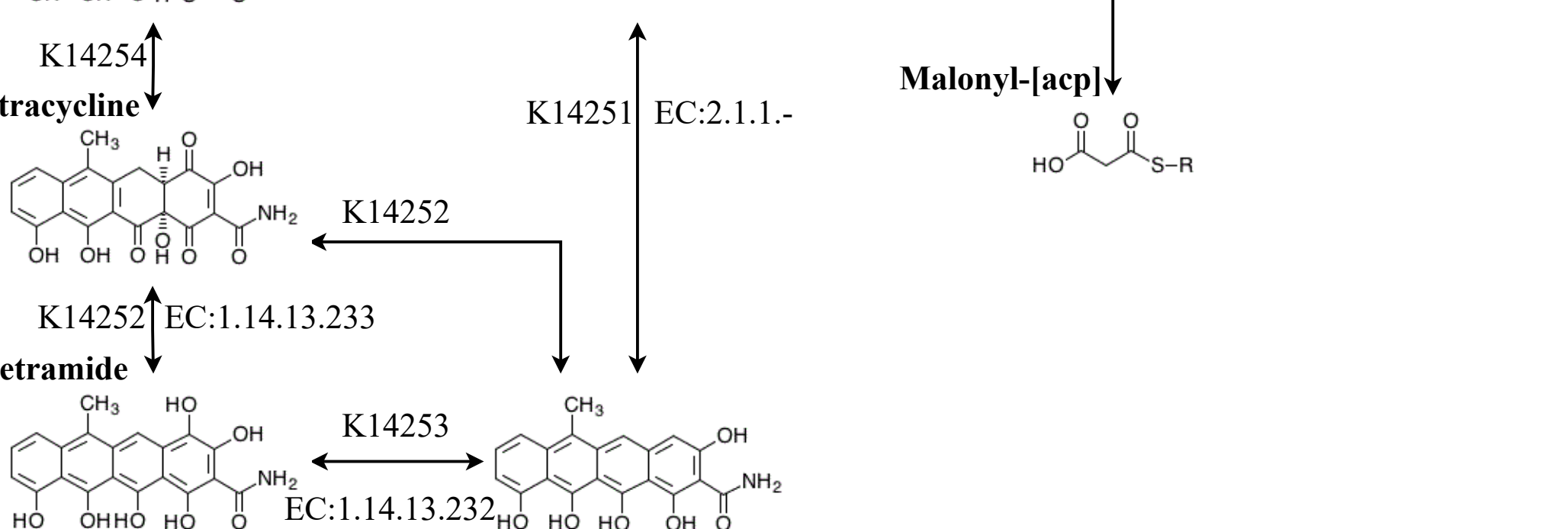
6-Methylpretetramide
