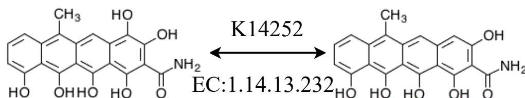
6-Methylpretetramide
