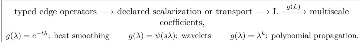
Figure 11.1: Spectral processing is downstream of edge identification. Different choices of g act on the same declared operator geometry but answer different multiscale questions.
