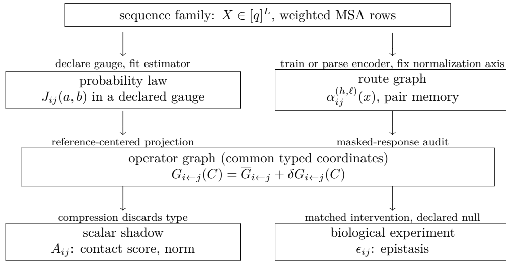
Figure 1.2: The spaces of this book on one page. Shared indices (i, j) appear in every box; the carried object differs. Only the operator-graph level holds both the fitted law and the audited model in common typed coordinates, and every arrow is a declared transformation whose lost or added assumptions the corresponding chapter makes explicit.
