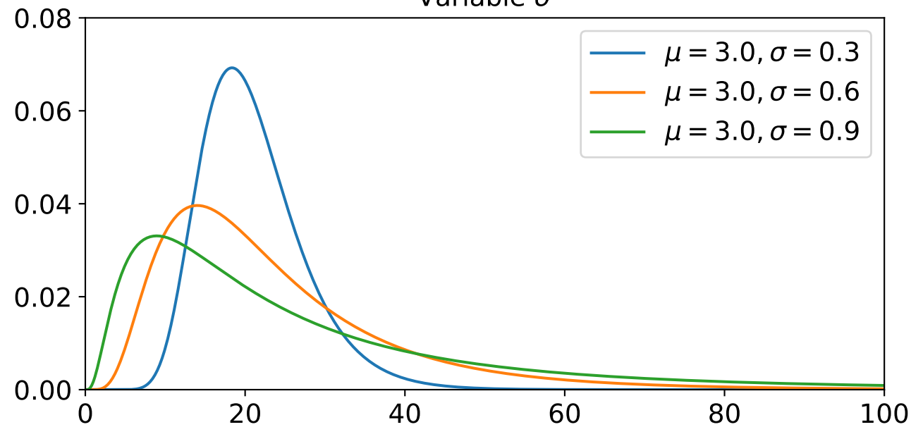
Variable \sigma
