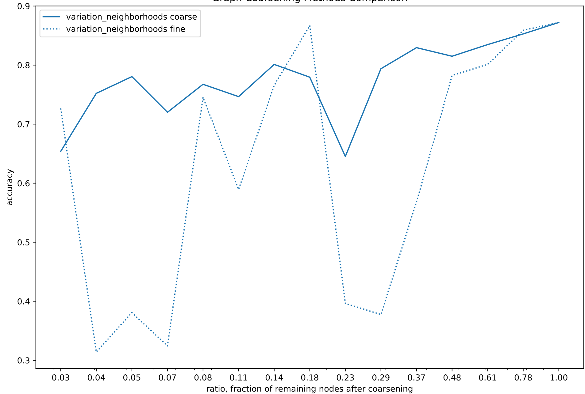
Graph Coarsening Methods Comparison
