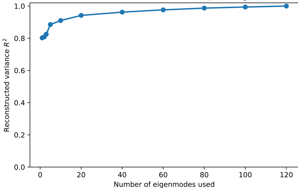
Cumulative BOLD reconstruction from spatial eigenmodes
