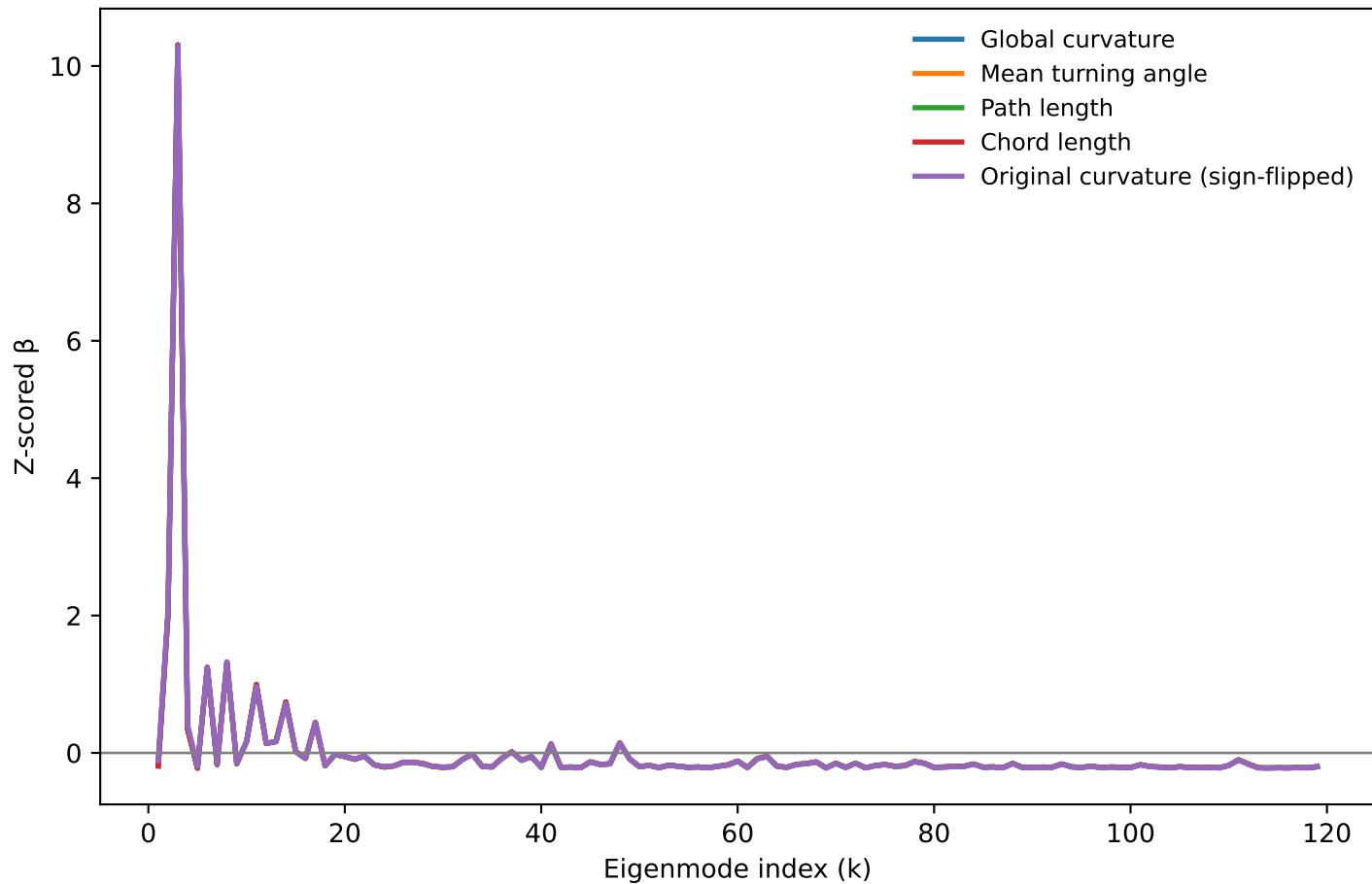
Normalized curvature family collapse
