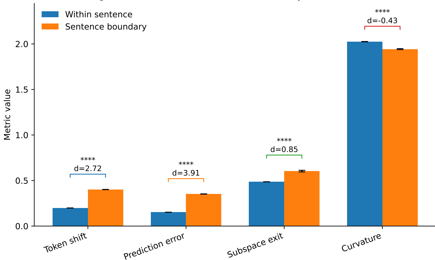
Linguistic transition metrics show boundary effects (Qwen3)
