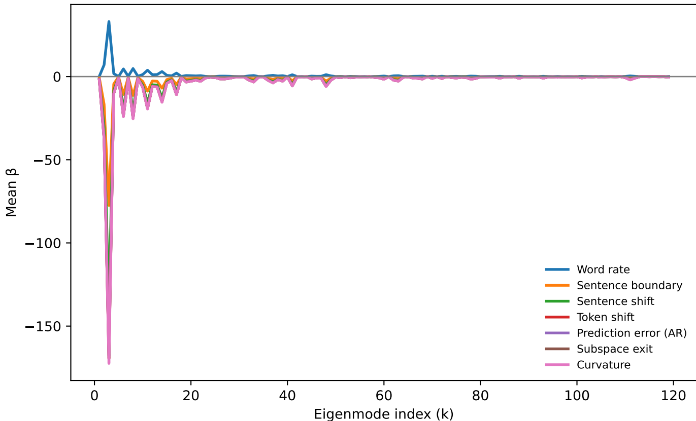
Word rate versus linguistic eigenmode profiles
