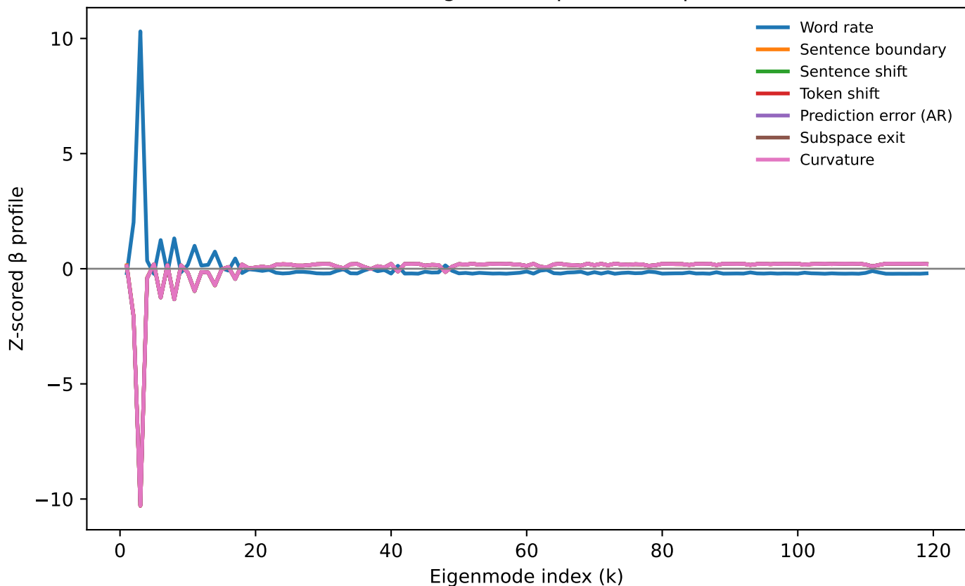
Normalized eigenmode profile comparison
