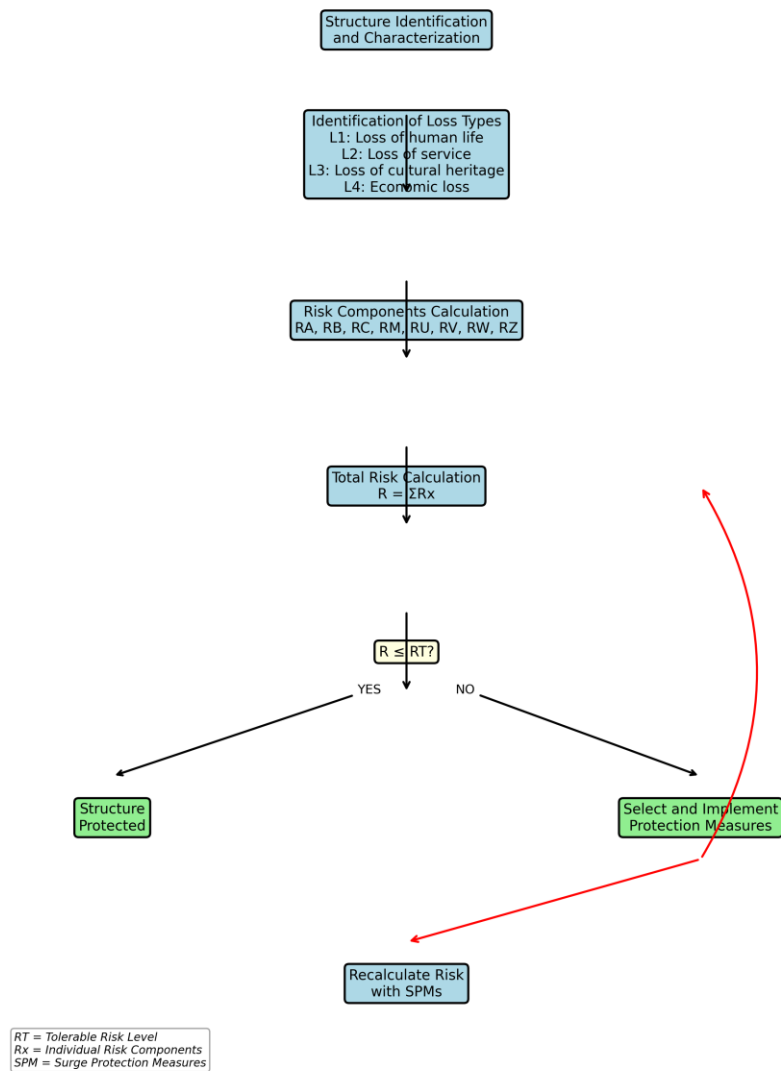
Figure 3: Risk Assessment Methodology per NBR 5419:2015 Part 2
