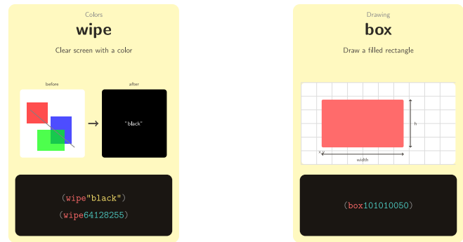
Figure 3: Reference cards for wipe (clear screen with color) and box (draw rectangle). Each card shows the function signature, a visual example on a grid, and the corresponding source code.
