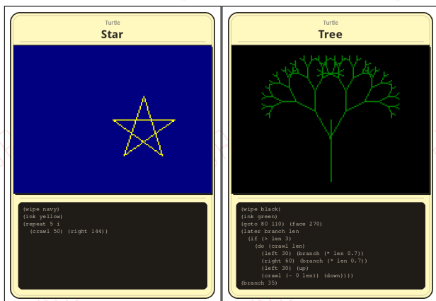
Figure 5: “Star” and “Tree” — turtle graphics cards.
