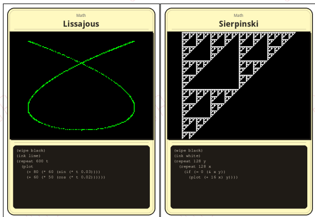
Figure 4: “Lissajous” (math curves) and “Sierpinski” (bitwise AND fractal).
