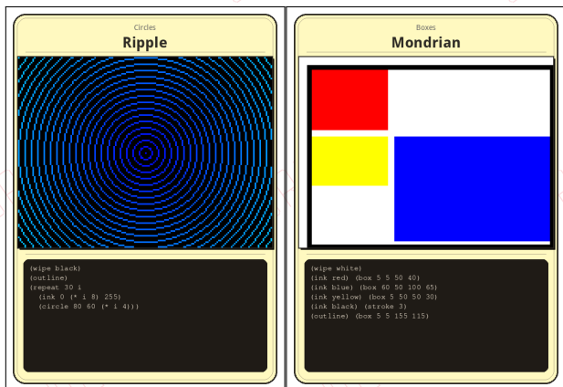
Figure 3: “Ripple” (circles) and “Mondrian” (boxes).
