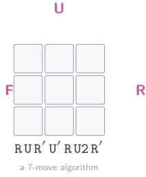
Figure 6: Singmaster’s cube notation [Singmaster, 1981]. Each capital letter names a face (Up, Down, Left, Right, Front, Back); a bare letter is a clockwise quarter-turn, a primed letter (′) a counter-clockwise quarter-turn, and a digit-2 a half-turn. The seven-token string R U R' U' R U2 R' is a complete algorithm portable between cubers, GitHub repos, and YouTube tutorials — the keymap-notation pair traveling as text.
