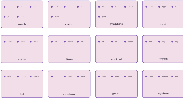
Figure 2: Twelve KidLisp categories with a sample of their built-ins. Each cell is a Category box laid out by the categories.style solver under a contains(c.box, f.dot) constraint per Member fact. Keys verified against kidlisp.mjs render in mono; absent keys (defined dynamically in the evaluator) are still listed but flagged in build output.
