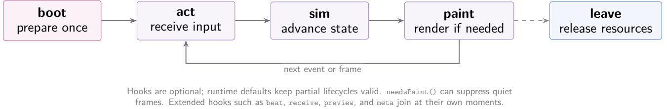
Figure 2: The runtime lifecycle is a score with optional movements. A piece may implement only the hooks it needs; the host supplies defaults, controls repainting, and performs cleanup when the work ends.
