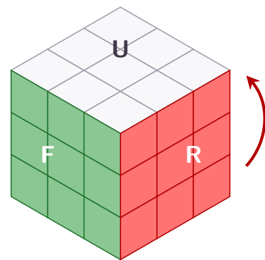
RUR'U'R'U2R' a 7-move algorithm
