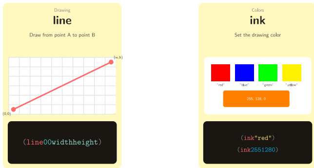
Figure 2: KidLisp line ink kidlisp.com/cards SVG
