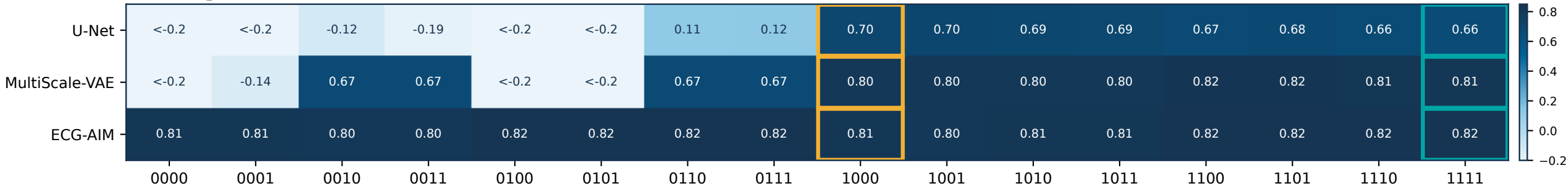
QRS correlation
