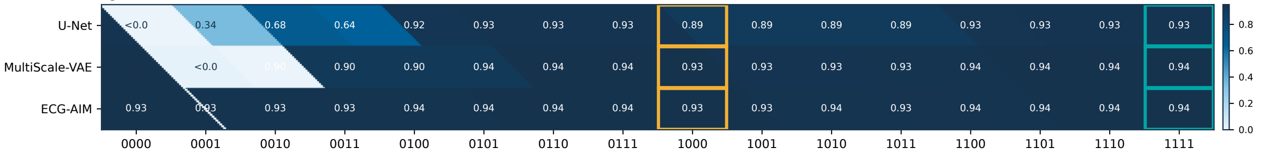
ST correlation
