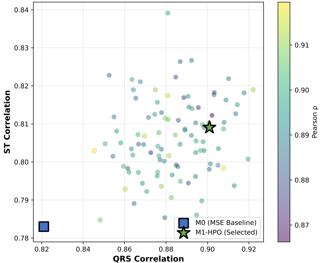
(B) Morphological Objectives
