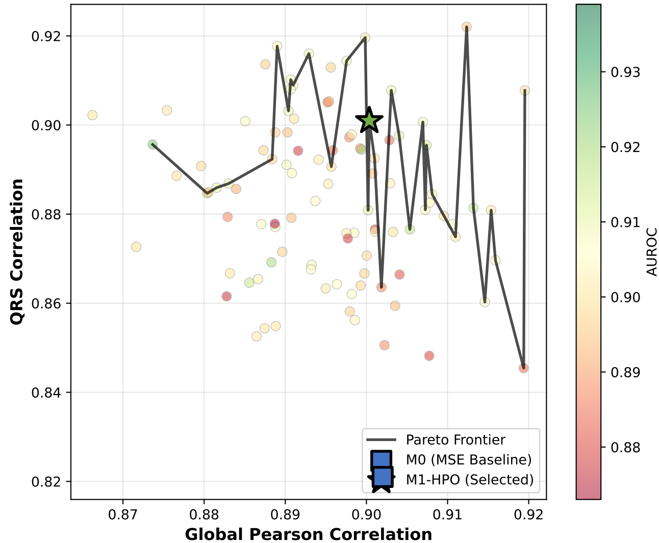
(A) Global Fidelity vs Morphology
