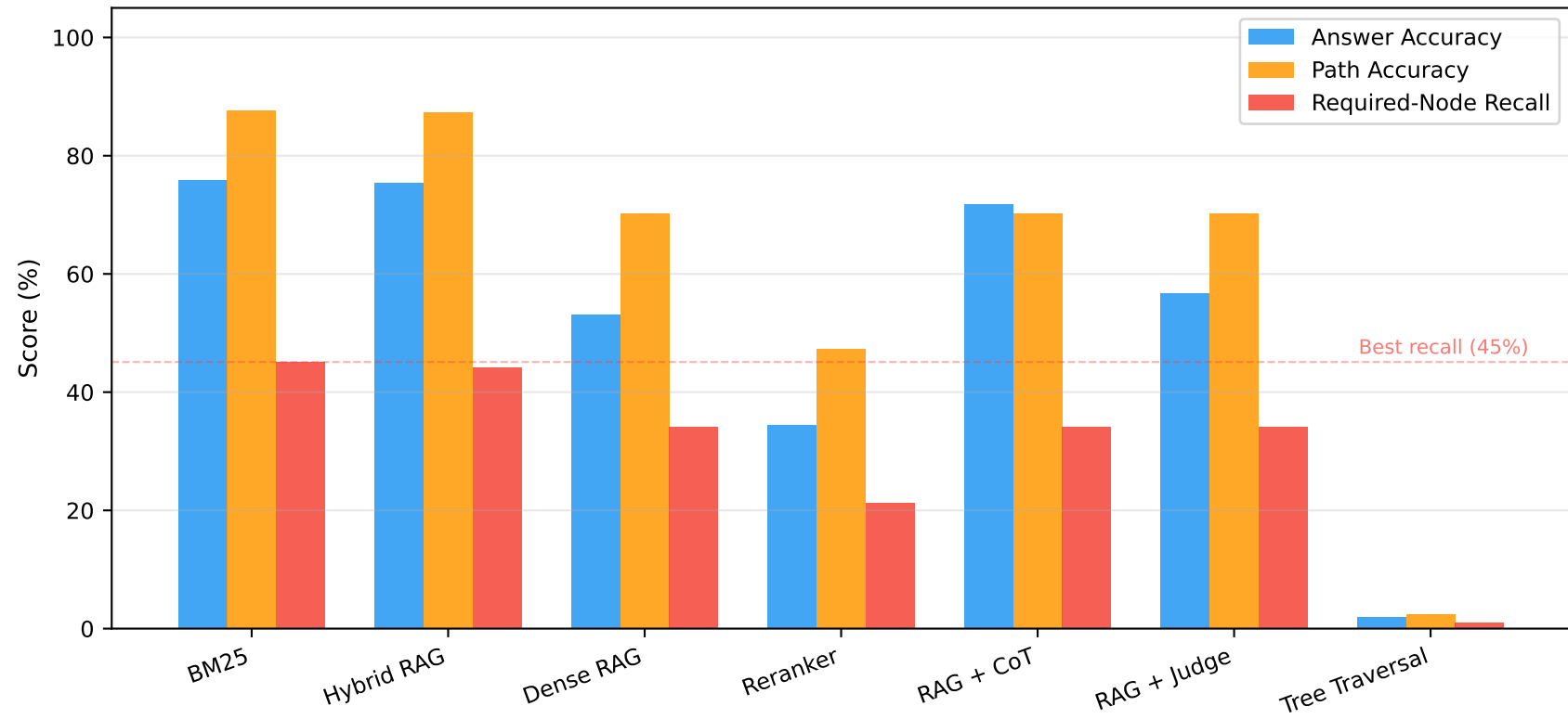
TreeBench-861: Method Comparison
