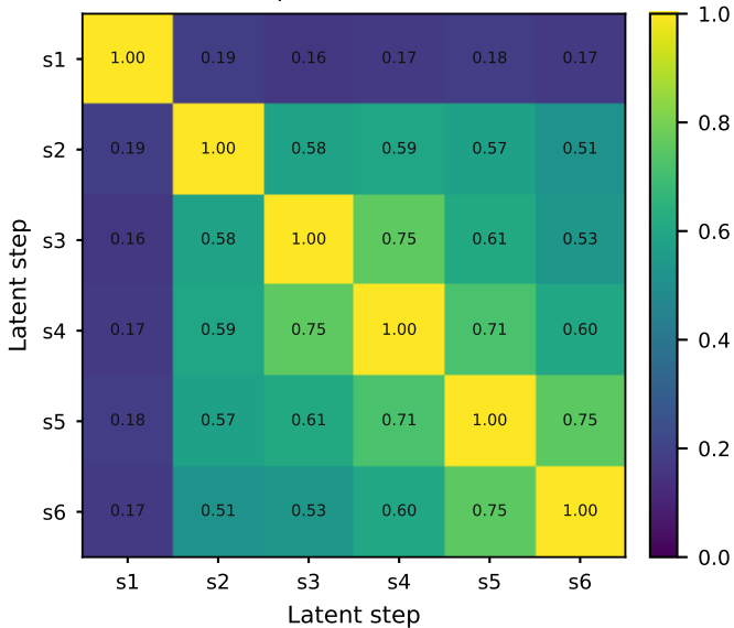
Latent-Step NMI (Baseline, k=32)
