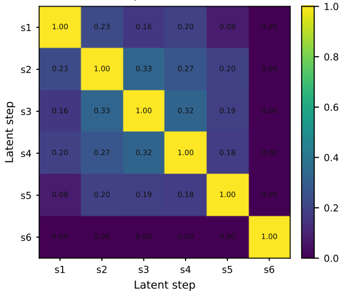
Latent-Step NMI (WIDER, k=32)
