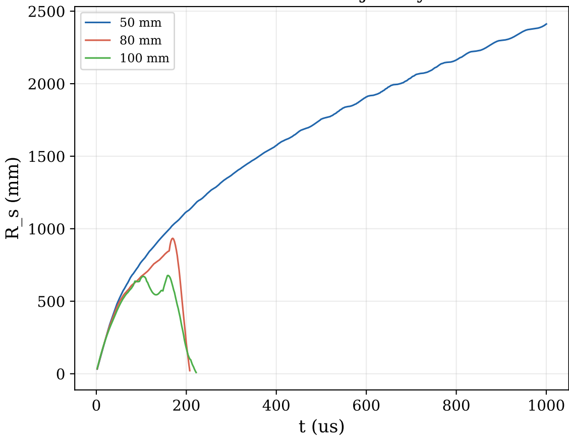
Shock front trajectory
