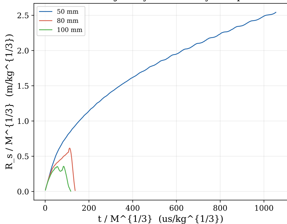
Shock trajectory — similarity collapse
