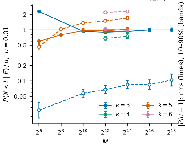
(a) p_F \approx 0.1 , one-sided signs; open, dashed: \Phi^{-1}(u) ; filled, solid: selection law at z_{sh} + \chi_{M-1}^2
