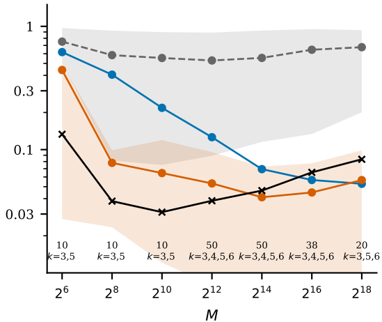
(b) cells with \rho^2 = 1 , p_F \in [0.03, 0.97] , u = 0.01 (cell count and k per M at bottom; not a paired sequence)
