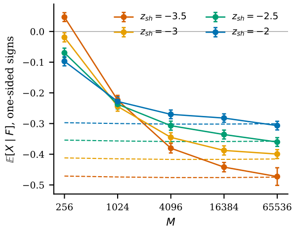
(a) k = 5 , all failures; dashed: selection law at z_{sh} (no fit)
