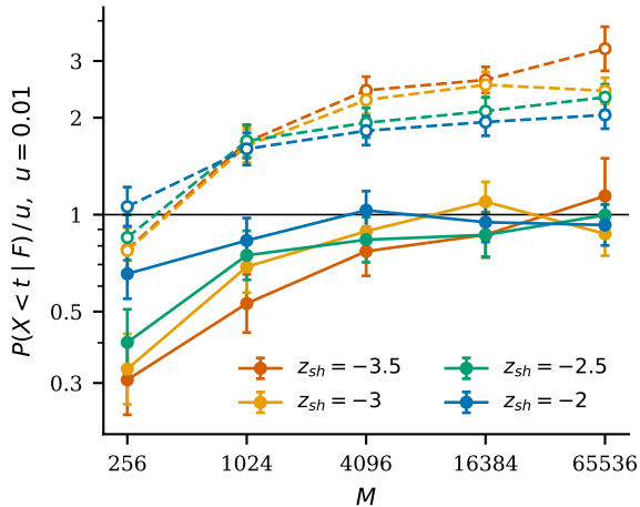
(a) k = 5 ; open, dashed: unconditional \Phi^{-1}(u) ; filled, solid: selection law at z_{sh} + \chi_{M-1}^2
