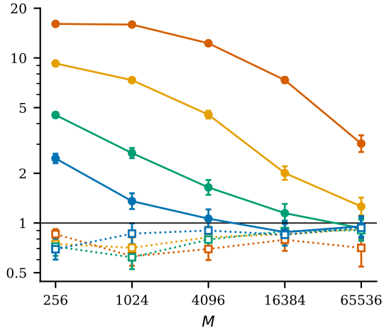
(b) k = 3 , selection law at z_{sh} + \chi_{M-1}^2 ; filled, solid: all failures; open, dotted: macroscopic-core failures only
