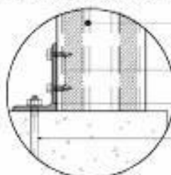
Bottom Fixing Detail
