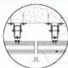
Horizontal Fixing Detail
