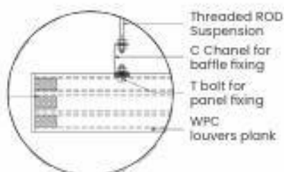
Typical Fixing Detail-A
