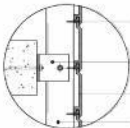
Typical Intermediate Detail
