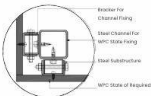
Horizontal Corner Detail
