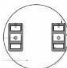
Horizontal Fixing Detail
