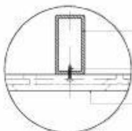
Typical Plain Detail
