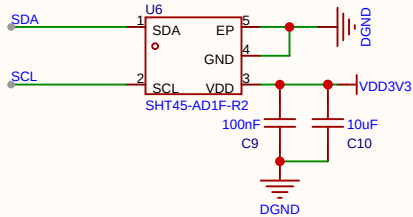
温湿度SHT45
