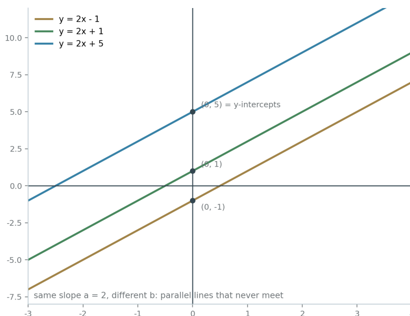
Figure 2.2: Same slope ( a = 2 ), different intercepts b - parallel lines that never meet.
