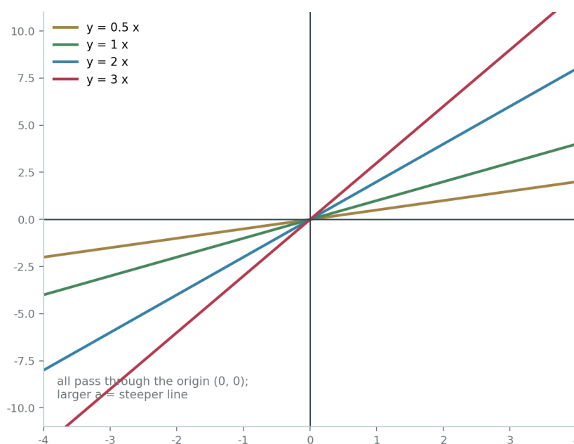
Figure 2.1: The family y = ax - all lines pass through the origin; larger a means steeper.
