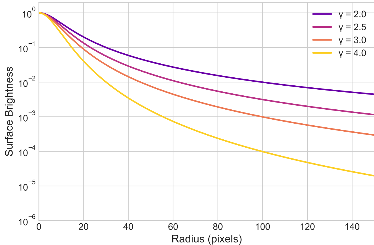
EFF Profile: Effect of Power-law Index
