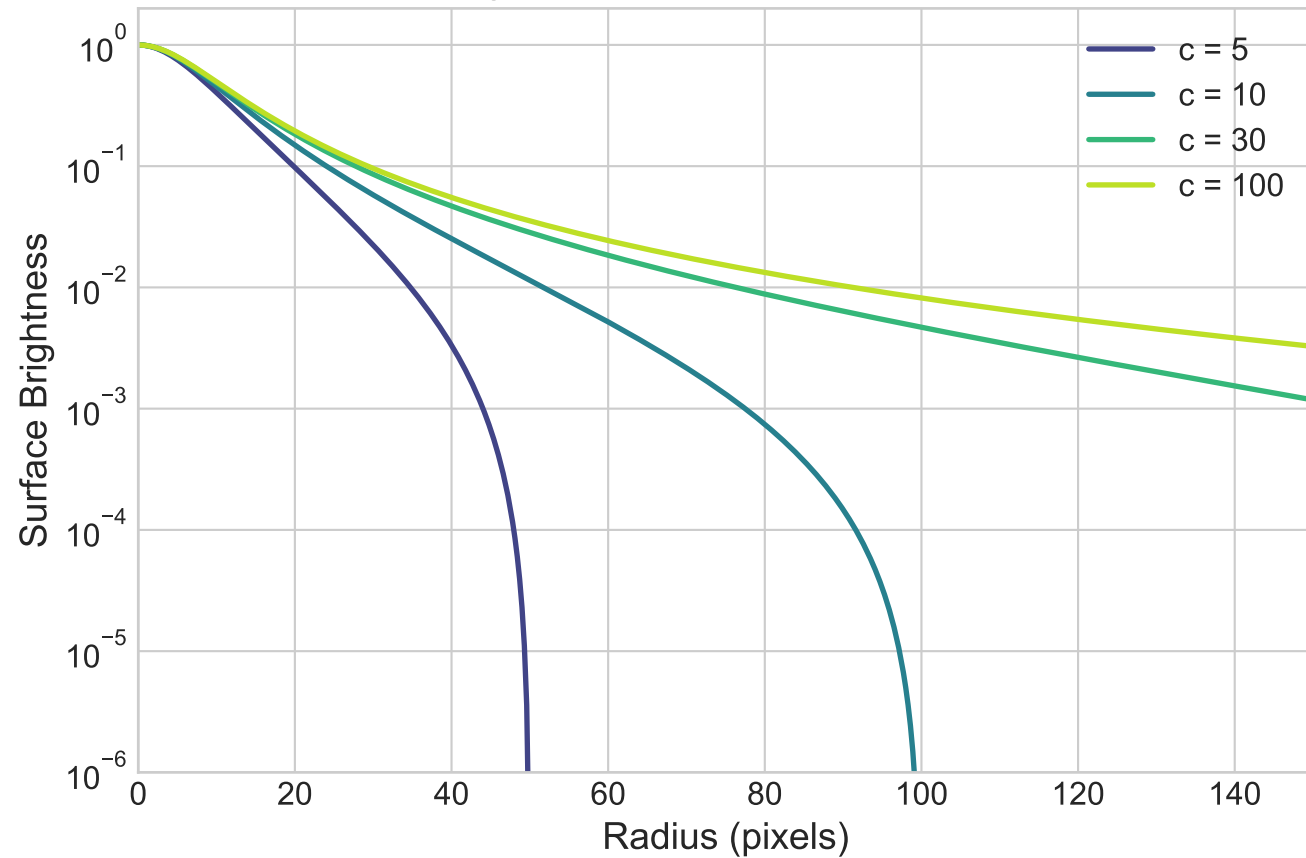
King Profile: Effect of Concentration
