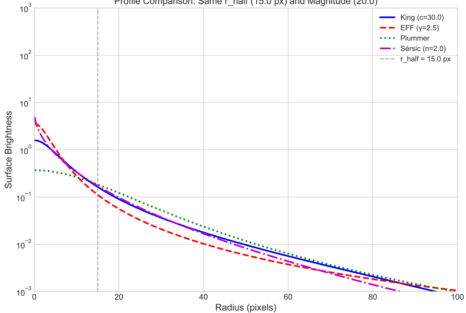
Profile Comparison: Same r_{\text{half}} (15.0 px) and Magnitude (20.0)
