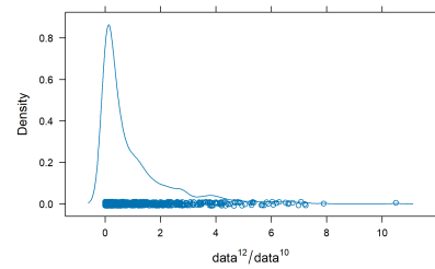
(b) Densityplot
