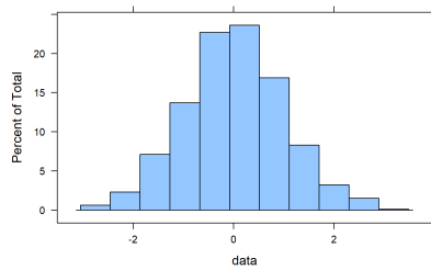
(a) Histogram
