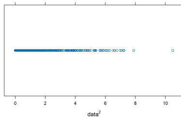
(c) Stripplot
