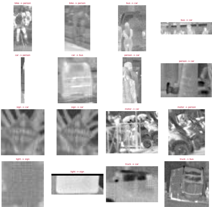
IR: Up to 2 Misclassified Validation Samples Per Class
