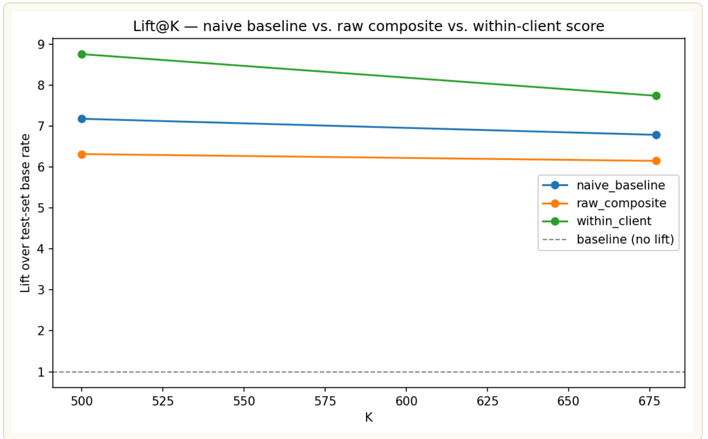
Figure 5 — Chart read: all three scores lead the impressions-only floor, but the within-client score leads the other two at K=500.
