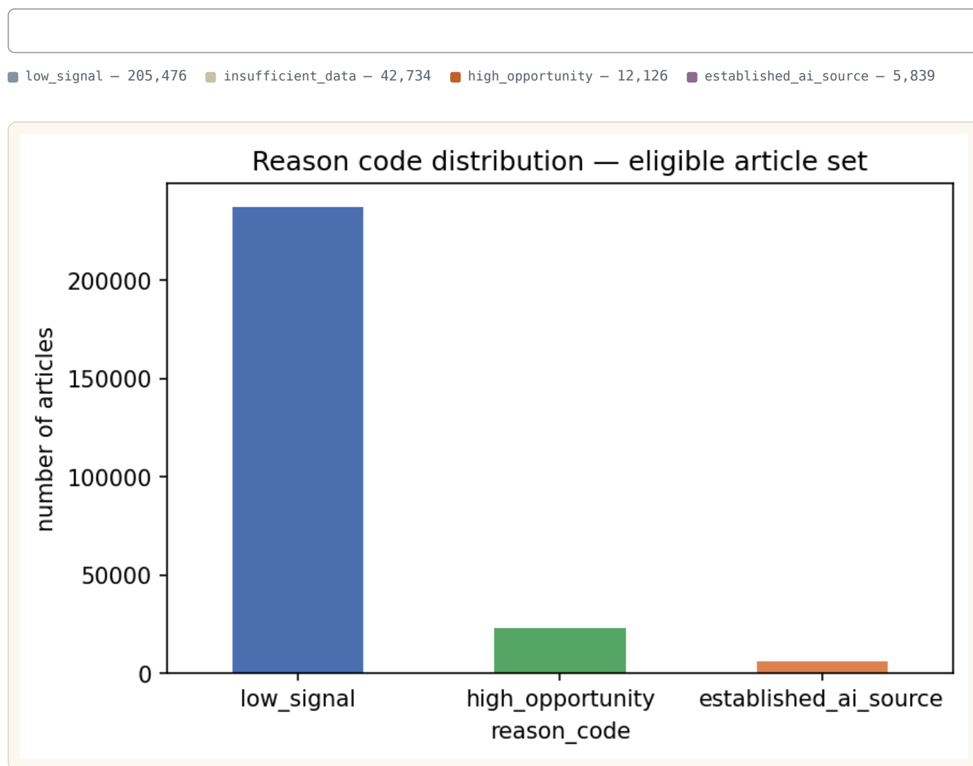
FIGURE 10 — Chart read: low_signal dominates by design — most articles simply aren't standout candidates in any given window.
