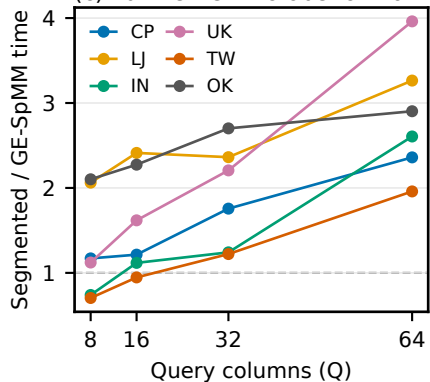
(c) Pull-kernel microbenchmark
