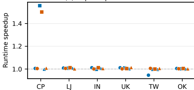
(c) In-place pull: propagation
