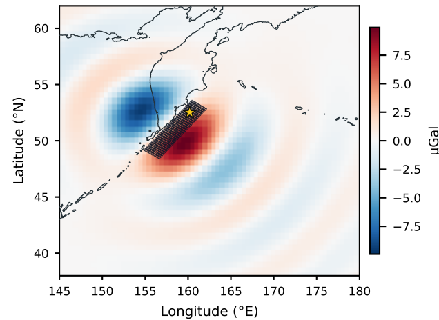
(e) USGS radial gravity (degree 60)
