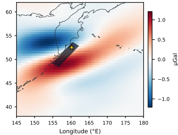
(g) USGS GRACE-FO-resolution radial gravity
