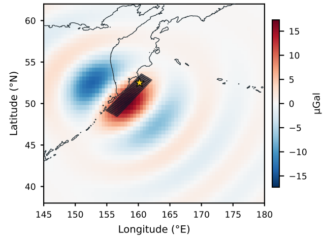
(b) GNSS radial gravity (degree 60)
