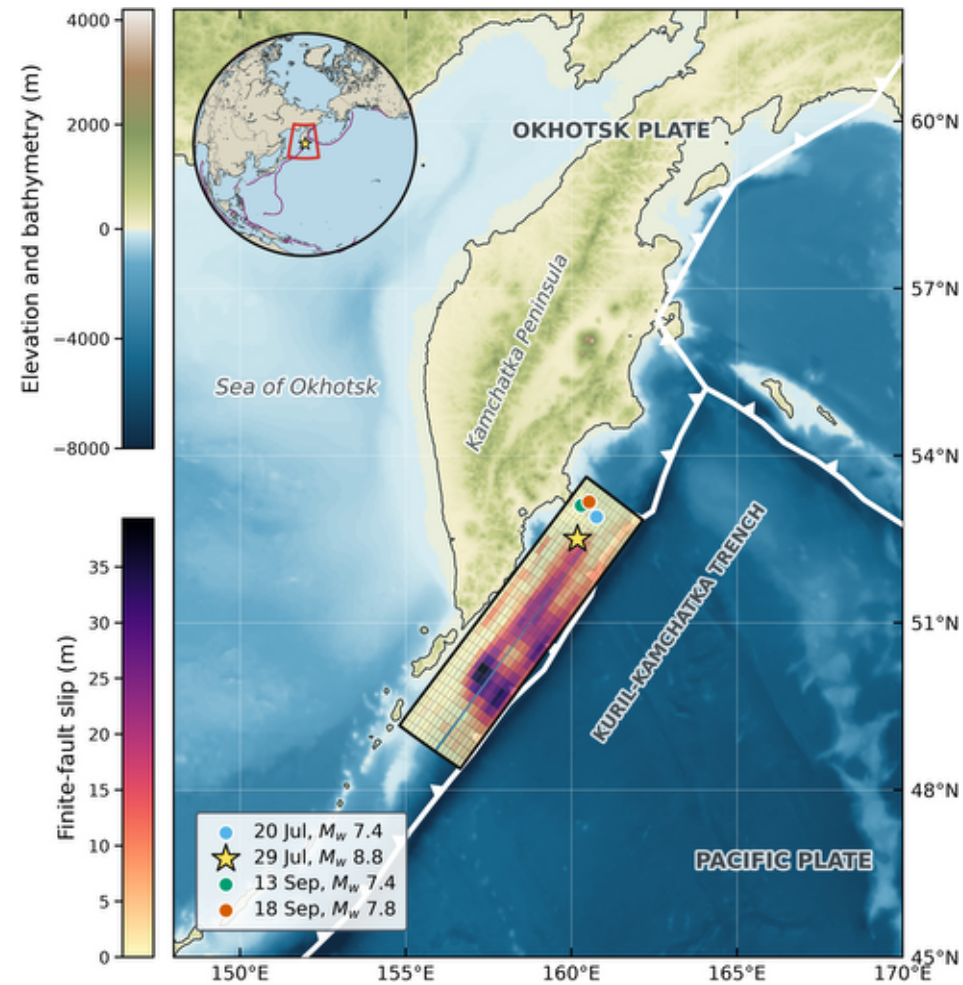
(a) Tectonic, bathymetric, and finite-fault setting
