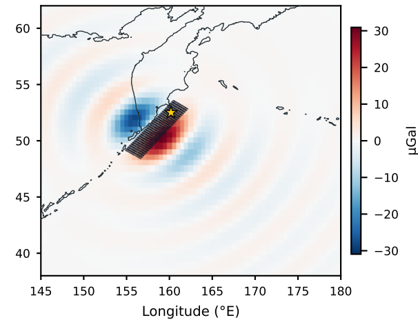
(f) USGS radial gravity (degree 96)
