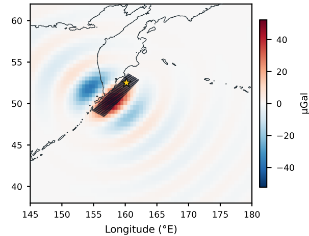
(c) GNSS radial gravity (degree 96)
