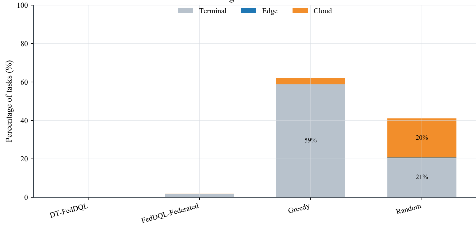
Offloading decision distribution
