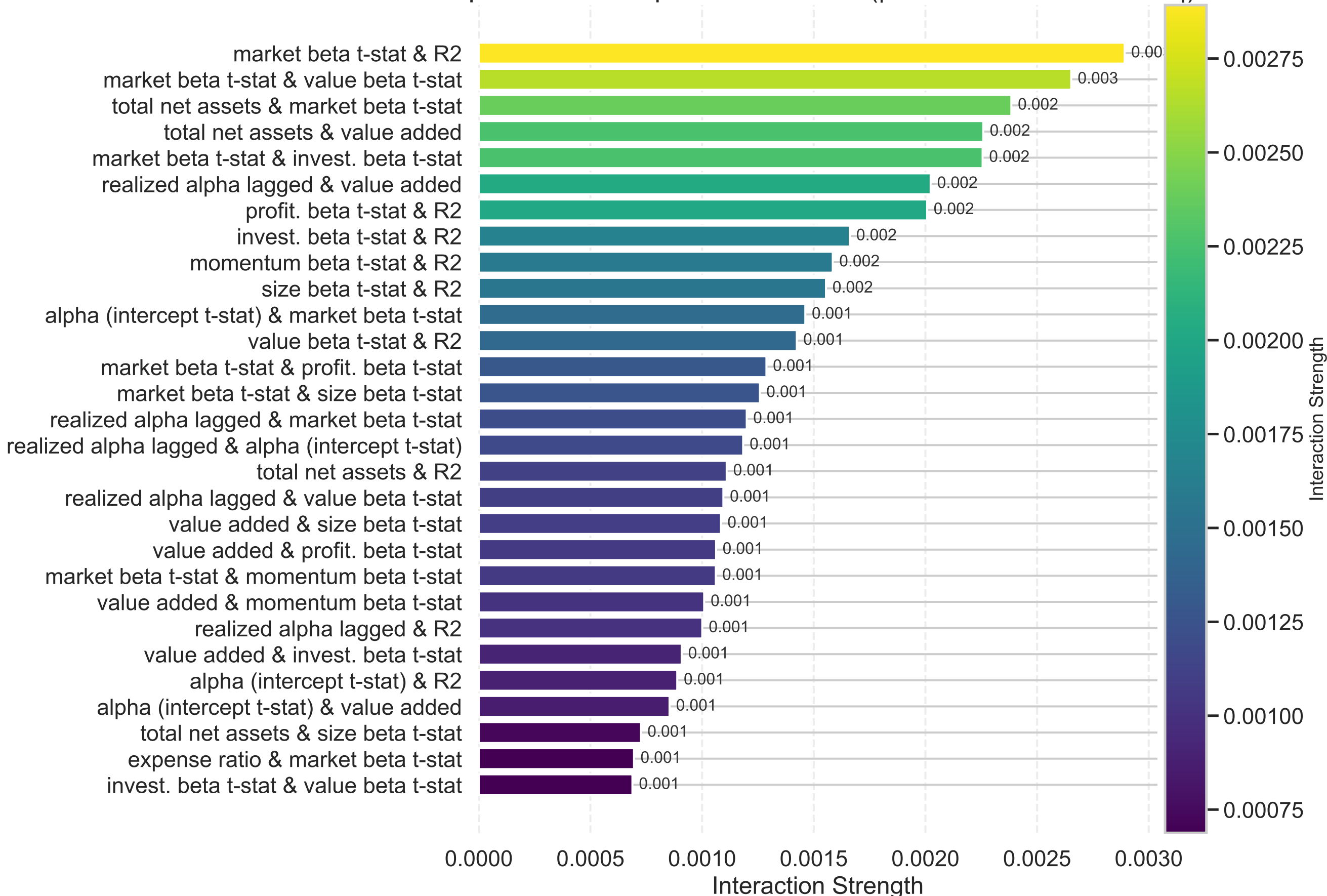
Top Interaction Importance — mean(|SHAP Interaction Values|)
