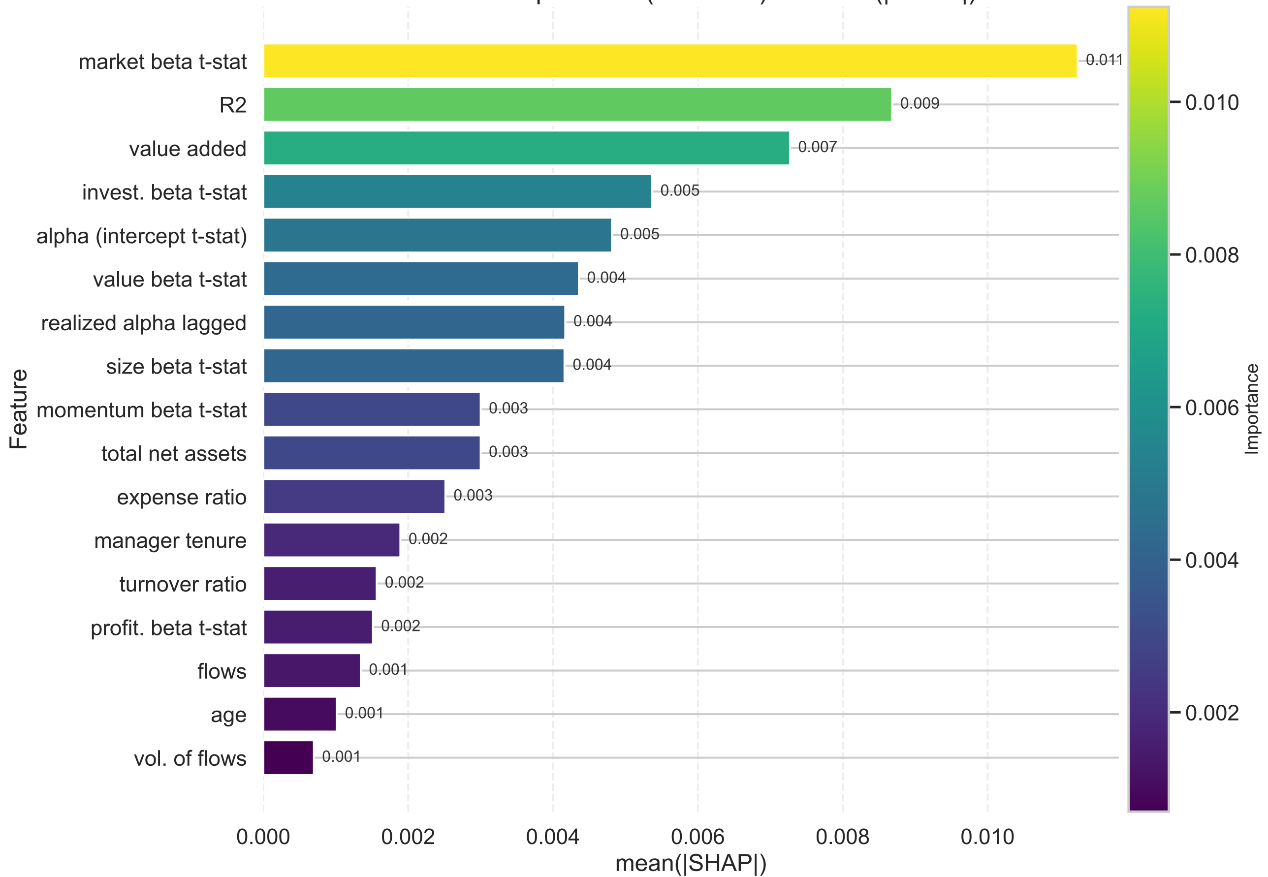
Variable Importance (XGBoost) — mean(|SHAP|)
