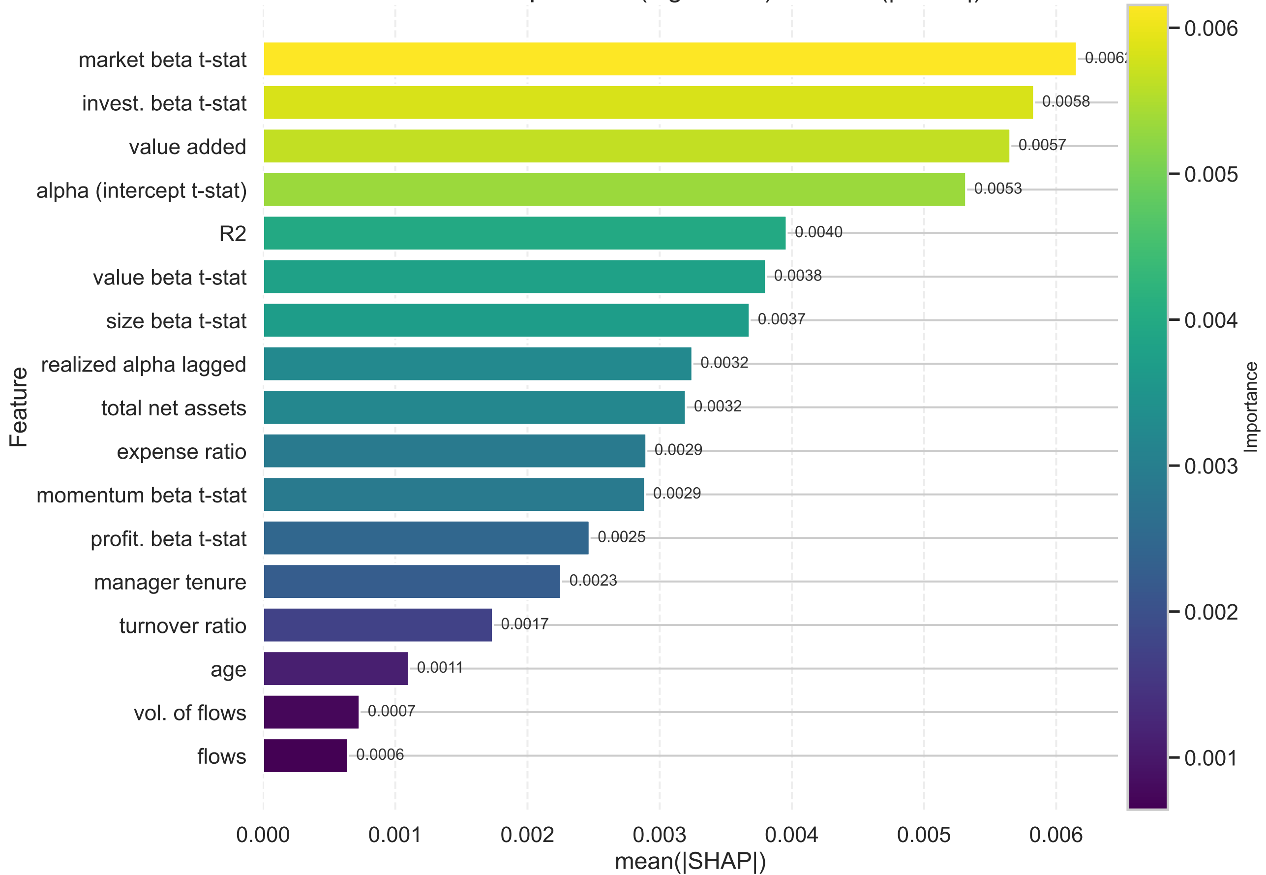
Variable Importance (LightGBM) — mean(|SHAP|)
