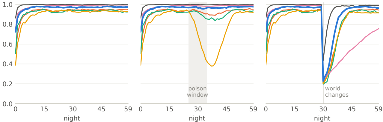
Self-report poisoning
